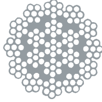
18X7 + IWRC (ROTATION RESISTING)
