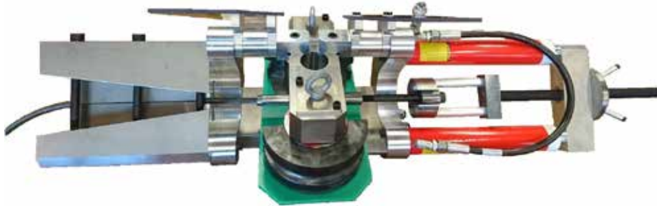
The Petersen P400 Combined Swage & Test Machine
