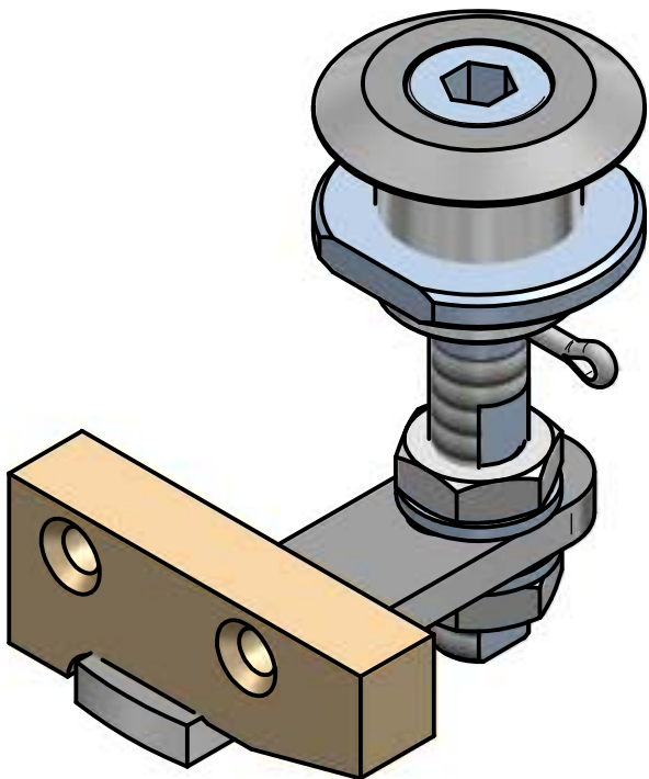
ISO VIEW
