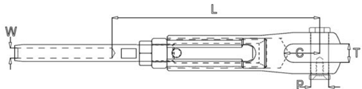
Compact Adjusters - Fork/Stud Long Adjustment
