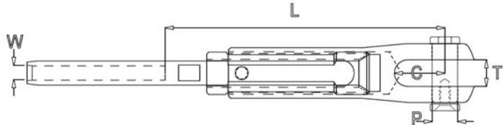
Compact Adjusters - Fork/Stud Short Adjustment
